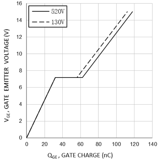
Fig. 14 Typical gate charge ( I_c=75A )
