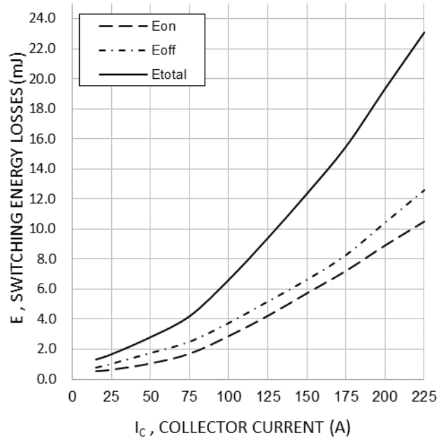
Fig. 10 Typical switching energy losses as a function of collector current (inductive load, T_{jy}=25^\circ C , V_{CE}=400V , V_{GE}=15/0V , r_G=8\Omega )
